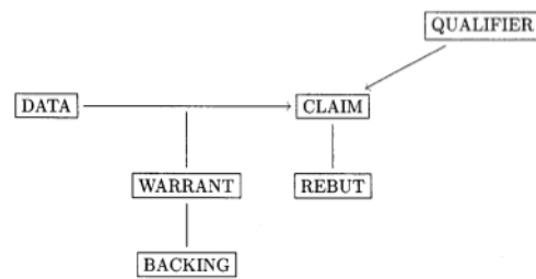
Fig. 2. An interpretation of Toulmin's argument pattern, from [43].
