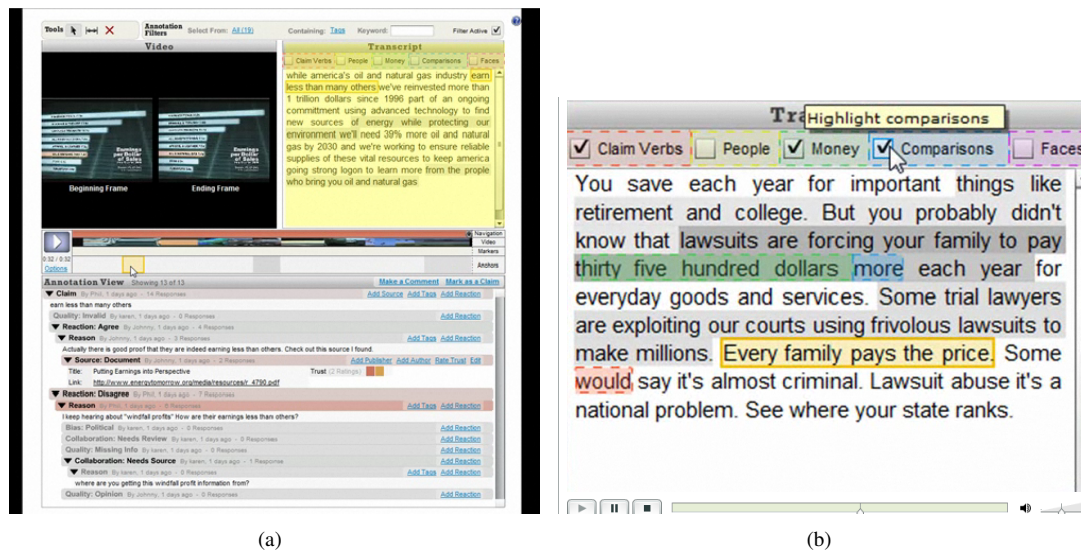
Fig. 53. Videolyzer (a) allows users to comment on the points made in a video; and (b) algorithmically determines segments of possible interest to help focus the discussion: in the transcript these are claim verbs and comparisons as well as mentions of people and money, and in the video these are peoples' faces.
