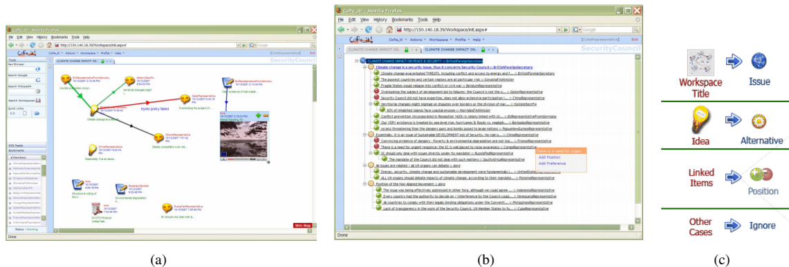
Fig. 39. CoPe_it! has (a) an informal spatial hypertext view; and (b) a formalized view, created by (c) automatically transforming items.
