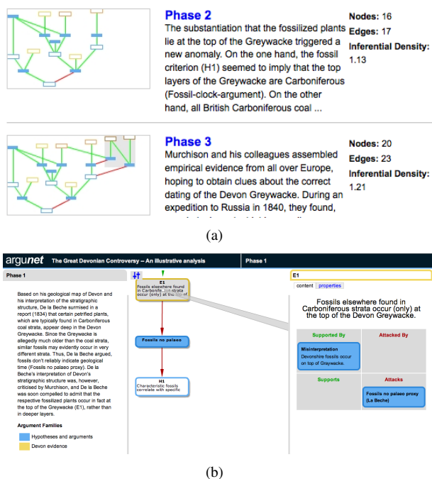
Fig. 29. Argumet can show an (a) overview of several related argument maps; and (b) in each individual map, nodes can be opened up to show arguments they support, attack, are supported by, and are attacked by.
